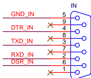
DB9_Female
